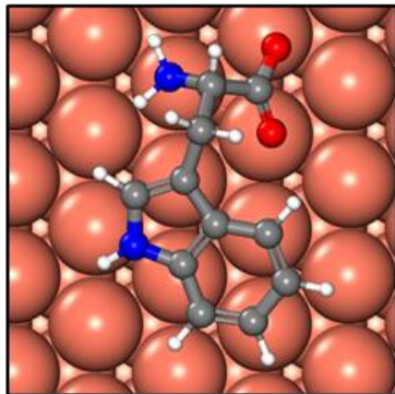
Trp-(111)
