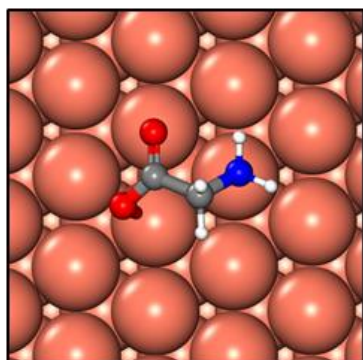
Gly-(111)
