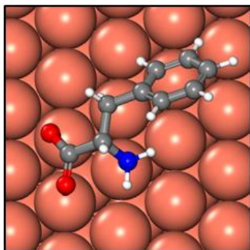
Phe-(111)
