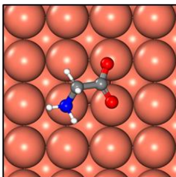
Gly-(100)
