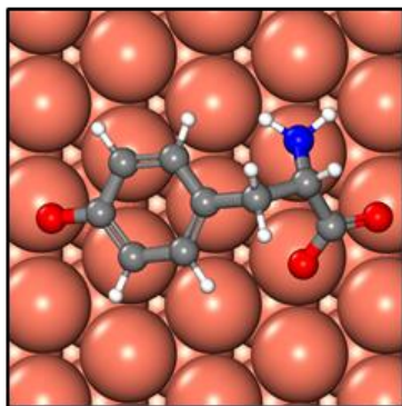
Tyr-(111)
