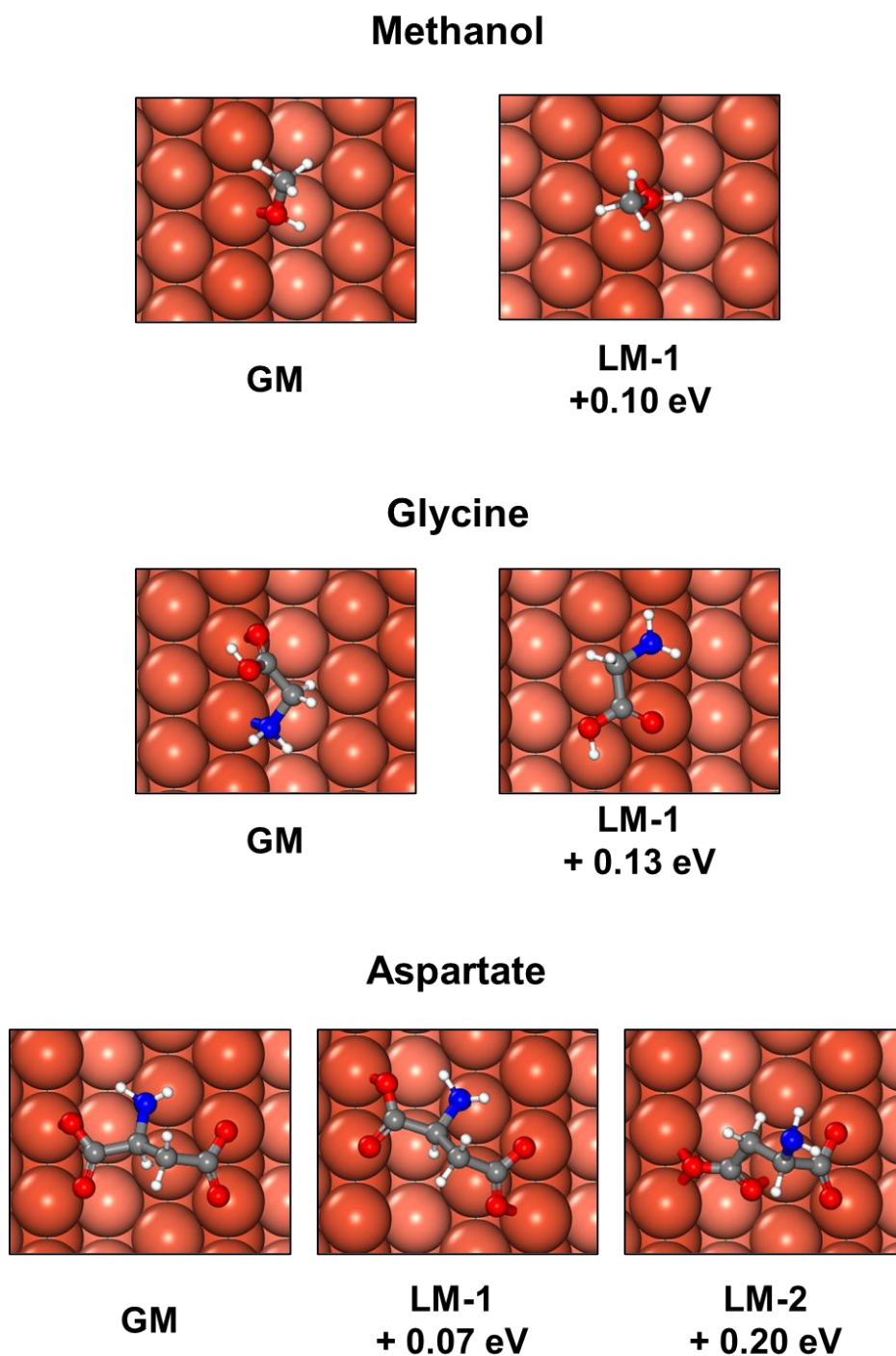
Figure S3. Representative adsorption structures for methanol, glycine, aspartate on Cu(211) surface. These adsorption structures and relative stability (using GM as reference) are predicted by AIMAP. The parameter settings are list in Table 1.
