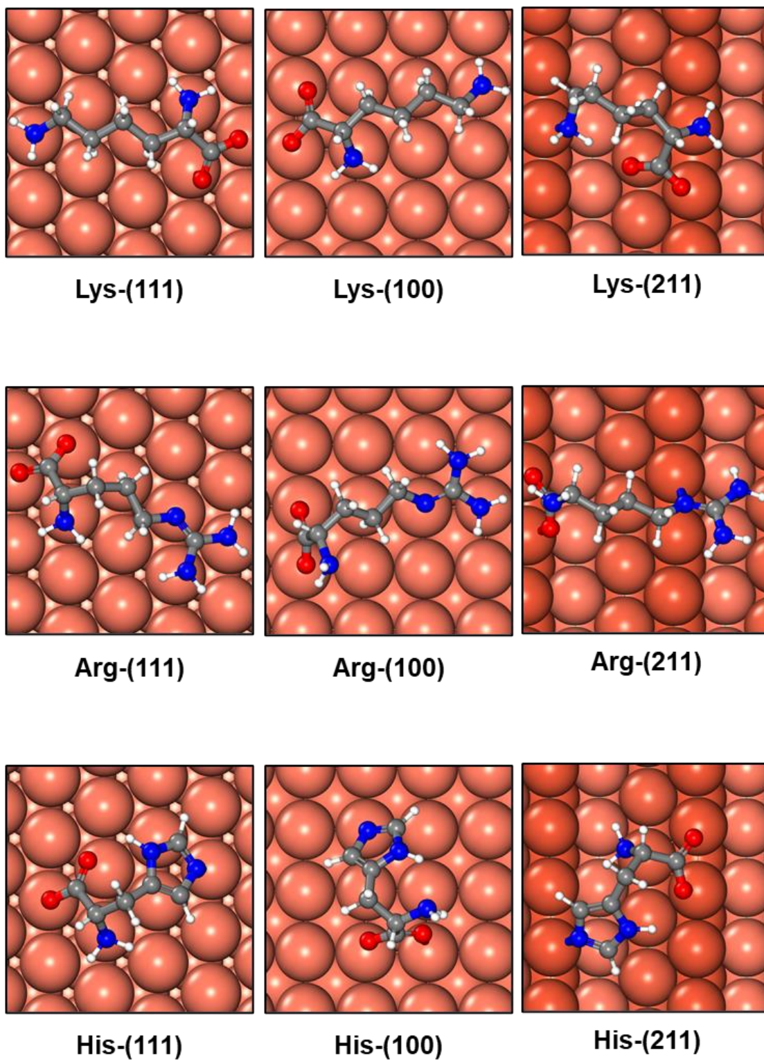
Figure S6.2 Adsorption structures of 18 types of AAs on achiral Cu(111), Cu(100), and Cu(211) surfaces.
