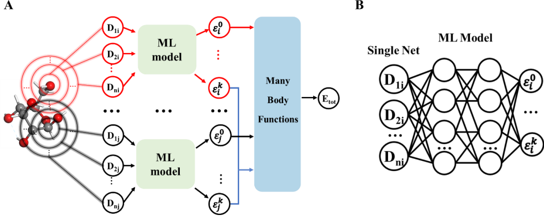
Figure S1. Illustration of the architecture of G-MBNN. A) Each atomic ML model (NN utilized in this work) outputs a series of coefficients \epsilon_i^k , which act as the parameters for different many-body functions. The total energy of system is written as the sum of many-body functions. B) The implementations of the ML model based on feed-forward NN.
