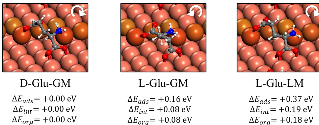
Figure S7.3. Adsorption structures of Glu on Cu(3,1,17) 5 surface. Indicated below each structure is \Delta E_{ads} , \Delta E_{int} , and \Delta E_{org} values (see text) using the most stable adsorption system as the reference. In the figure, the white cycle arrow highlights the chirality recognition, following the sequence of amino \rightarrow carboxylate \rightarrow side chain.
