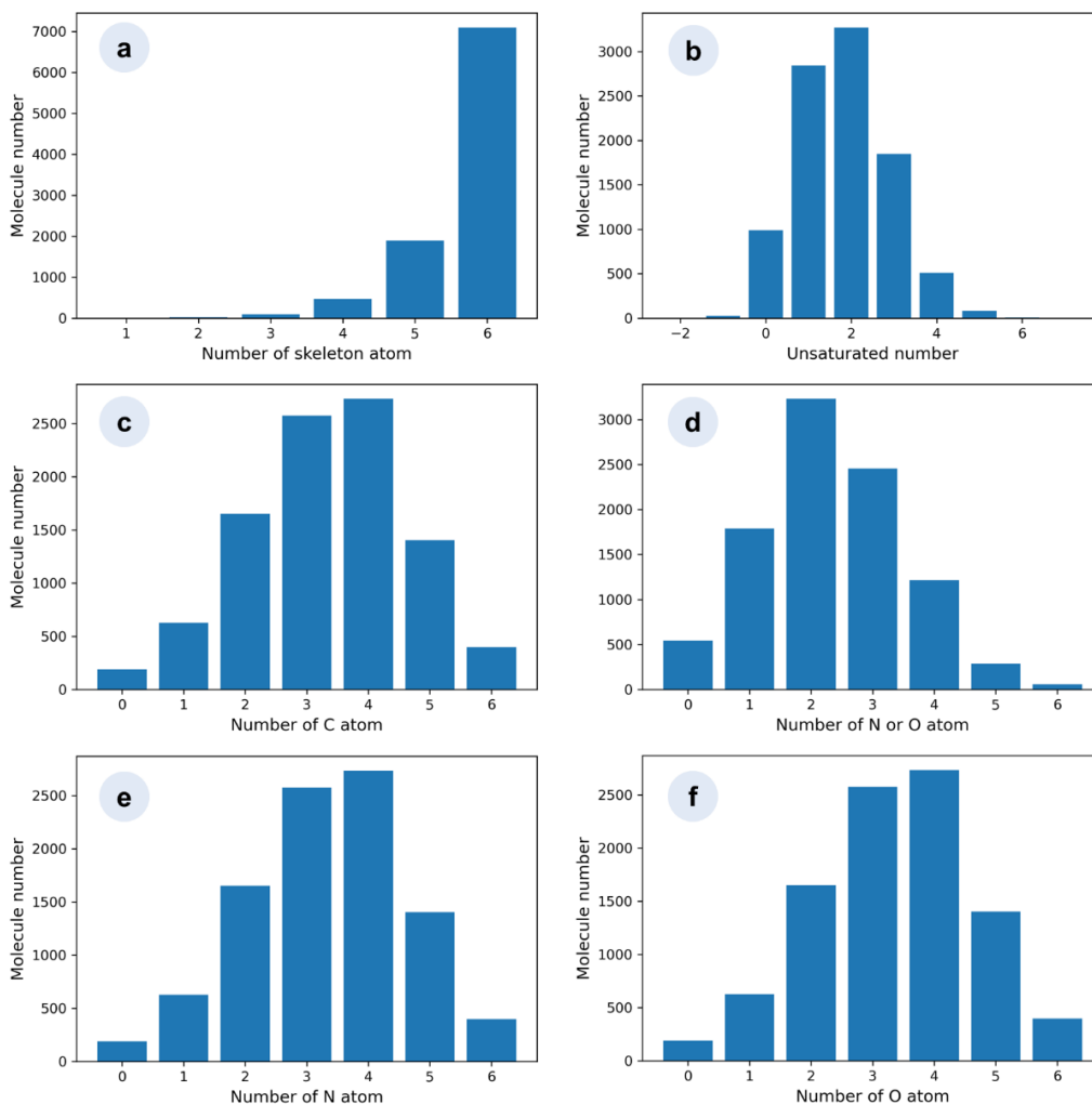
Figure S4.2 Molecule compositions in the Cu-HCNO6 database. These histograms depict the distribution of molecules with specific compositions from the Cu-HCNO6 database. The number of molecules is categorized by (a) The number of skeleton atoms (C, N, and O); (b) The value of the unsaturated number (calculated by: (2 \times n(C) + n(N) - n(H))/2 - 2 , n(C), n(N), n(H) represent the number of respective elements) (c) The number of carbon atoms; (d) The number of nitrogen or oxygen atoms; (e) The number of nitrogen atoms; (f) The number of oxygen atom.
