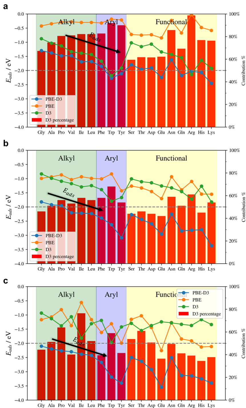
Figure S6.1 Adsorption energy of 18 types of AAs on Cu(111), Cu(100), and Cu(211) surfaces. The three sub-figures depict the adsorption energy decomposition for (a) Cu(111), (b) Cu(100), and (c) Cu(211) surfaces. The calculated adsorption energy using PBE-D3 is represented by blue dots, while its decomposition into contributions from PBE and D3 dispersion correlation is shown by yellow dots (PBE) and green dots with red bars (D3). A black arrow highlights the increasing of adsorption energy with side chain volume for amino acids with alkyl side chains.
