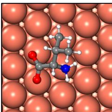
Val-(111)
